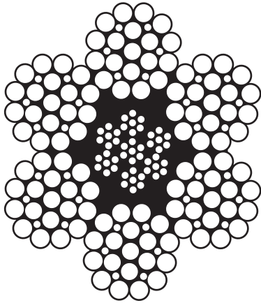
6 X 25 Extra Improved Plow Steel Construction
