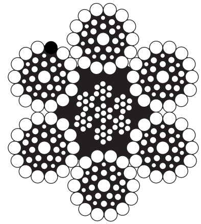
6 X 37 3/4" Extra Improved Plow Steel Construction
